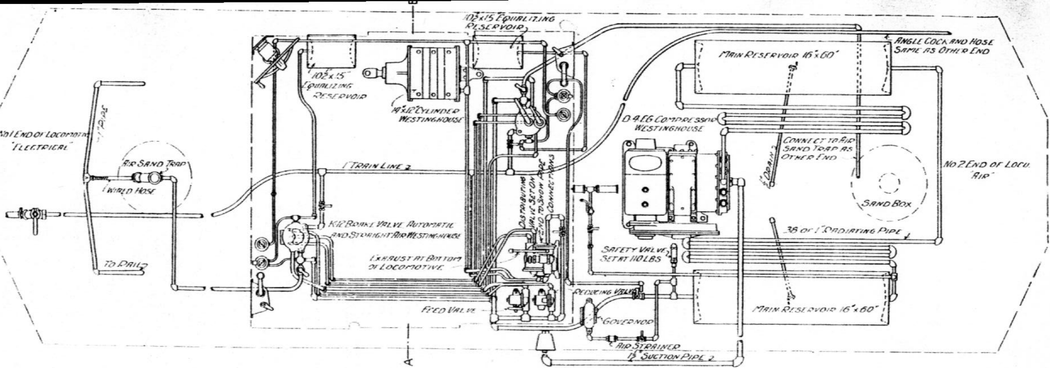
Illinois Traction Locomotives—Plan of Braking Installation.
