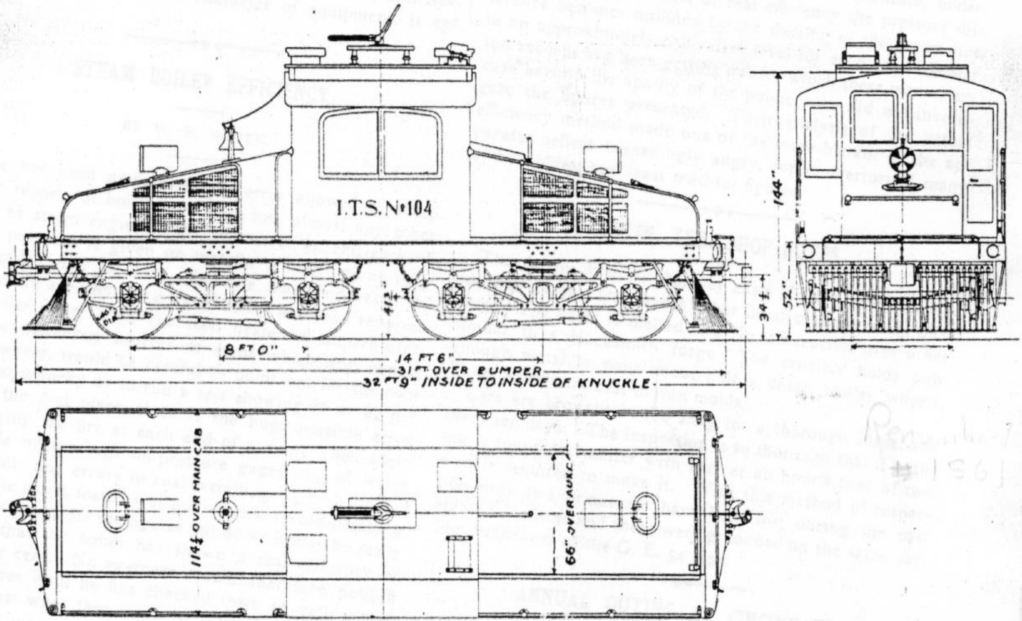
FIG. 27.—50-TON LOCOMOTIVE EQUIPPED WITH FOUR G E A-609 MOTORS
