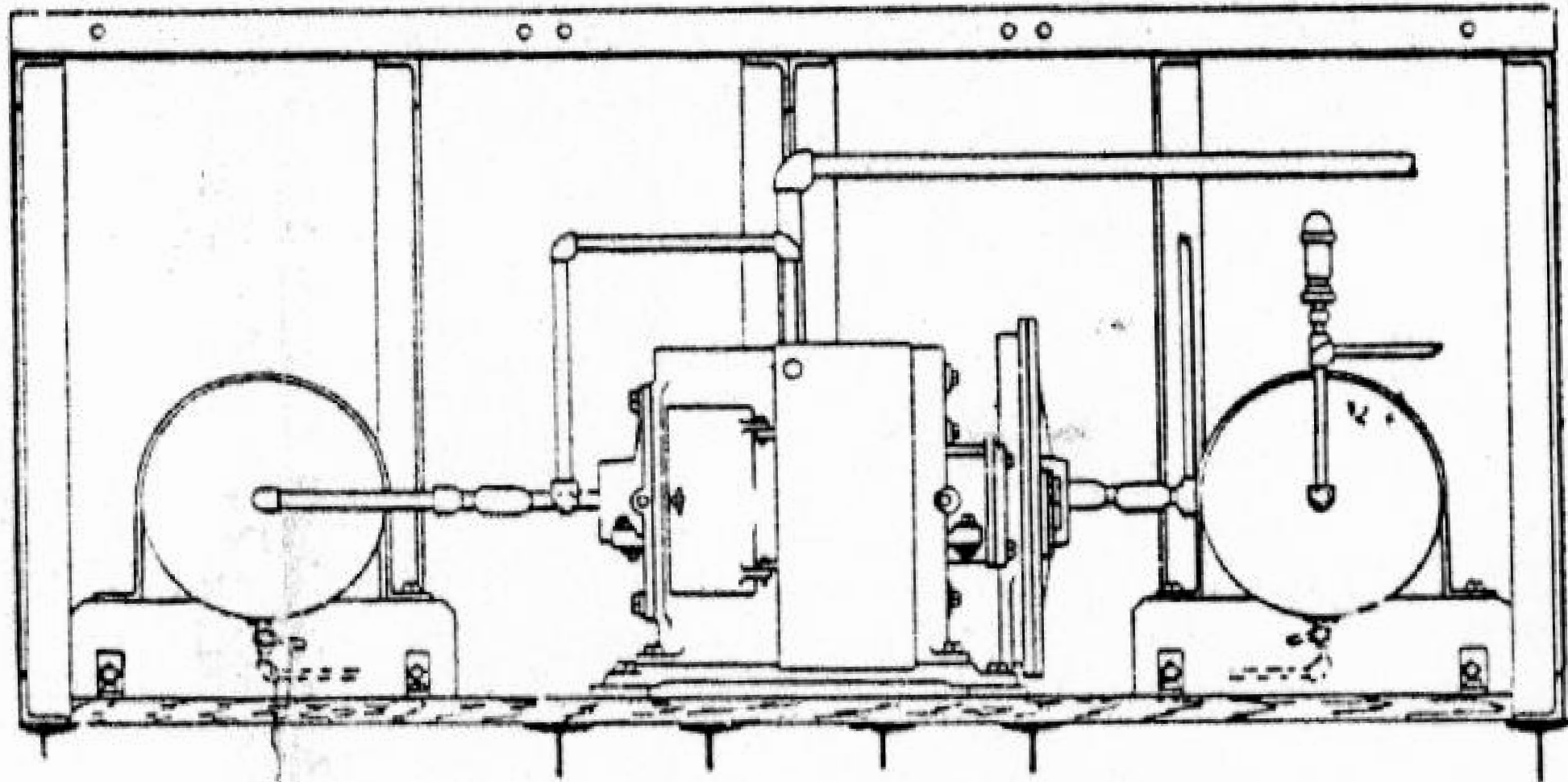
Illinois Traction Locomotives—Section at End Door.
