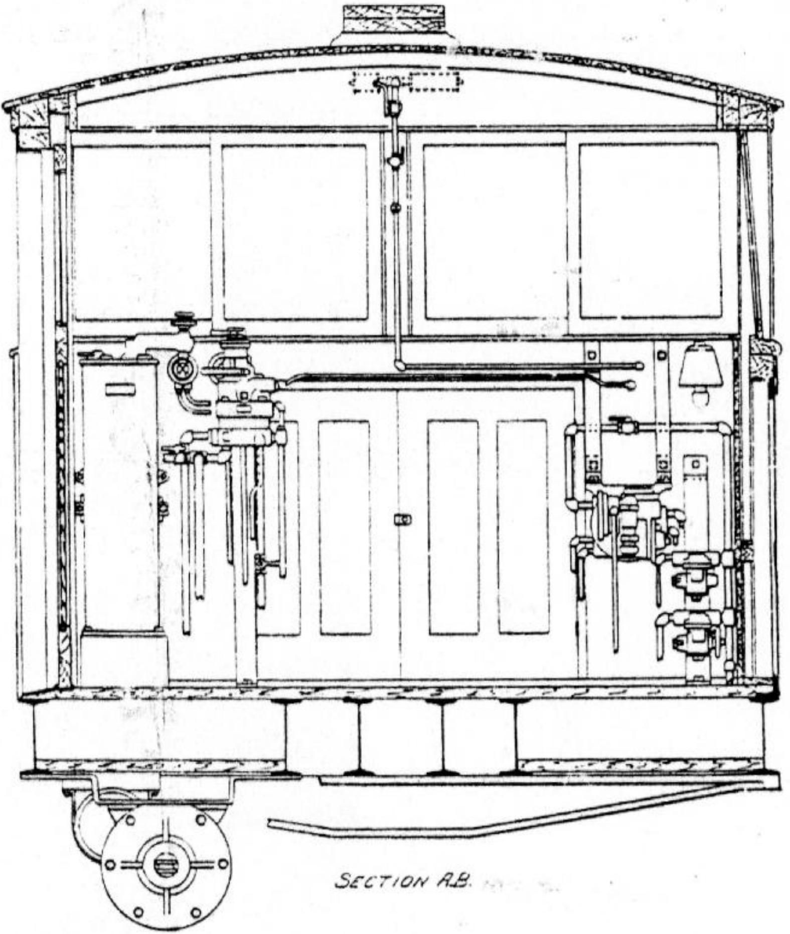
Illinois Traction Locomotives—Sectional Elevation Through Cab.
